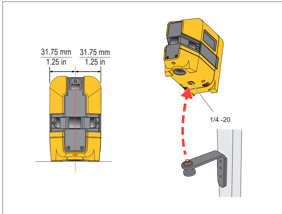
Figure 1. Center Point and Accessory Mount
