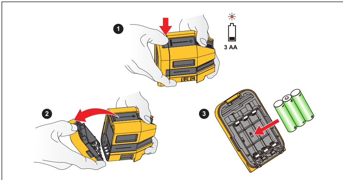
Figure 8. Battery Replacement
