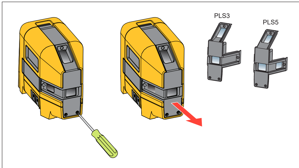
Figure 9. Housing Glass Insert Replacement
