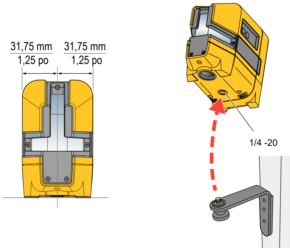
Figure 1. Point central et support d'accessoires
